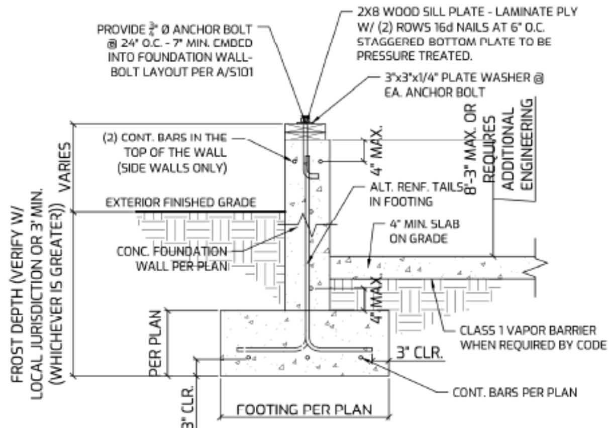
1 TRIO BASEMENT SIDE WALL EXT. CONTINUOUS FOOTING
