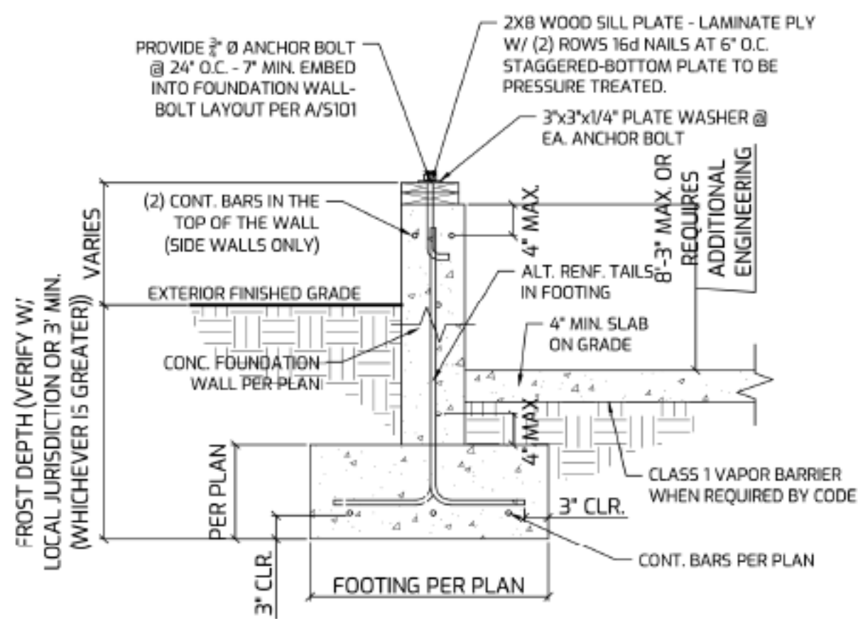
1 TRIO BASEMENT SIDE WALL EXT. CONTINUOUS FOOTING
