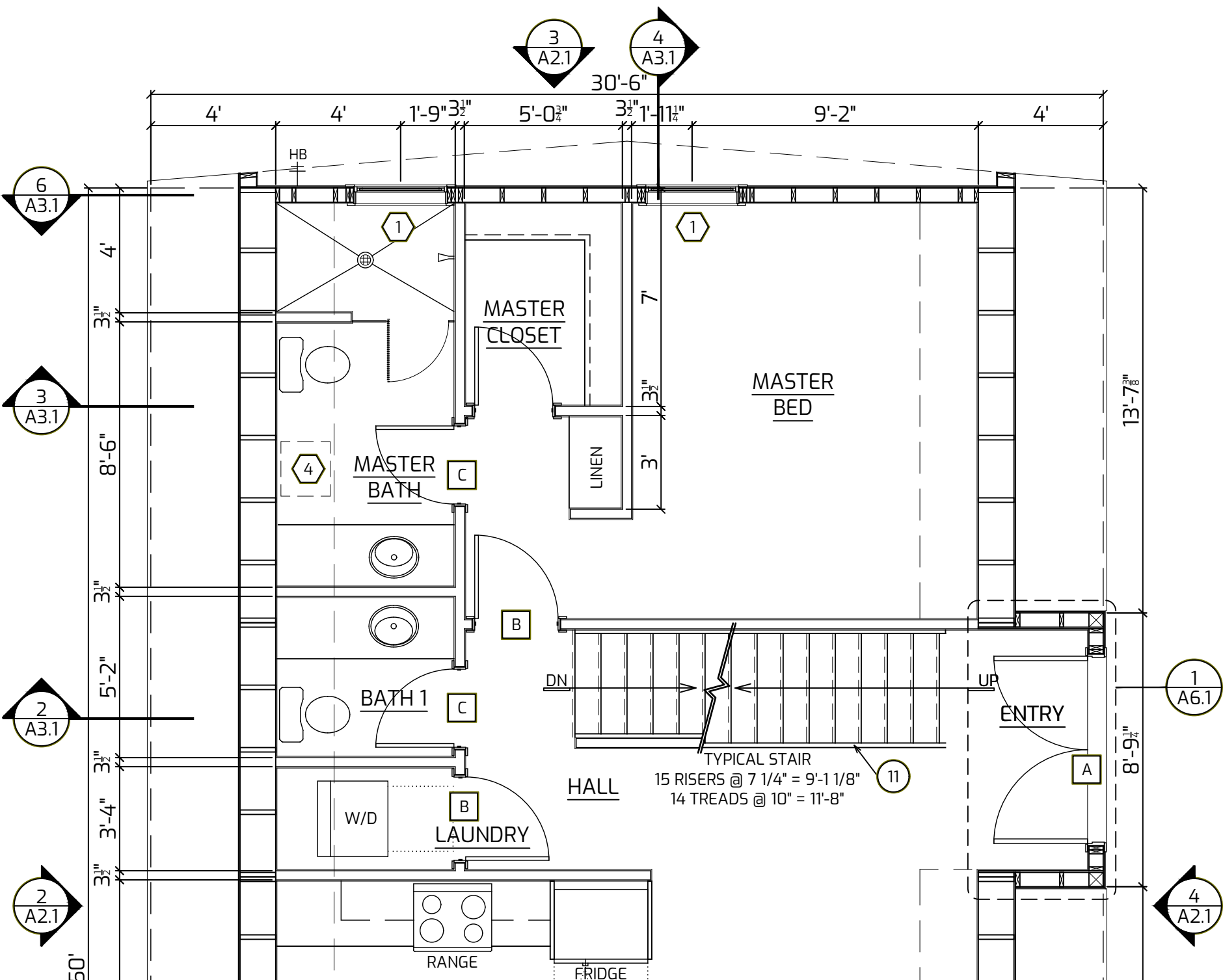
1 TRIO 150 PRIMARY BEDROOM SUITE OPTION "A" 1/4" = 1'-0"
