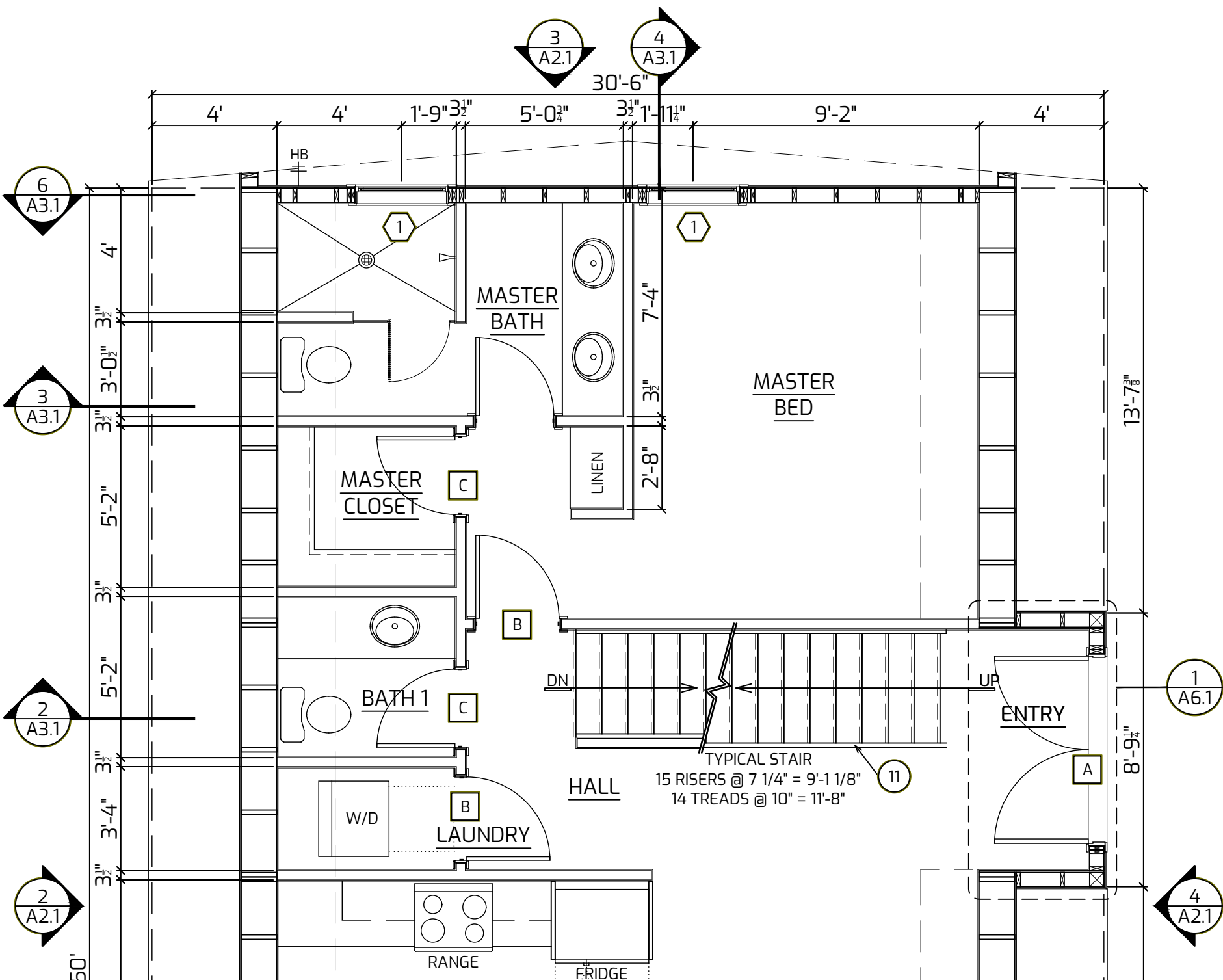
3 TRIO 150 PRIMARY BEDROOM SUITE OPTION "B" 1/4" = 1'-0"
