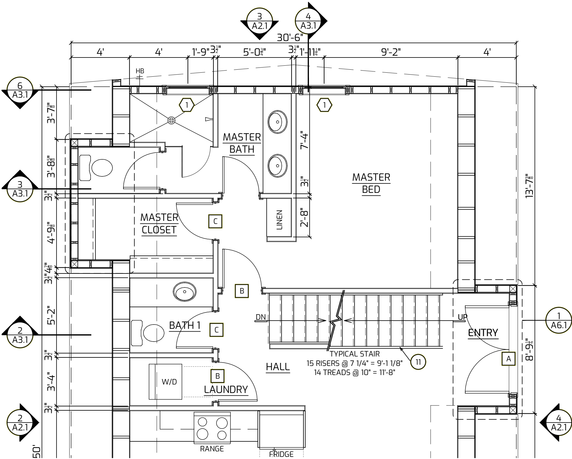
4 TRIO 150 PRIMARY BEDROOM SUITE OPTION "B" W/ DORMER 1/4" = 1'-0"
