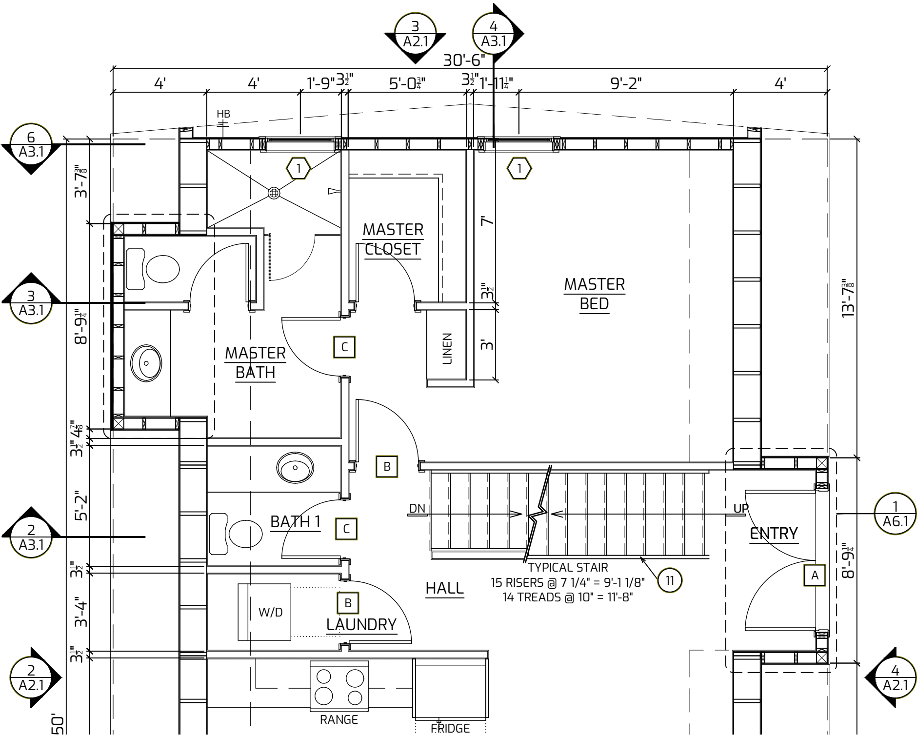
2 TRIO 150 PRIMARY BEDROOM SUITE OPTION "A" W/ DORMER 1/4" = 1'-0"
