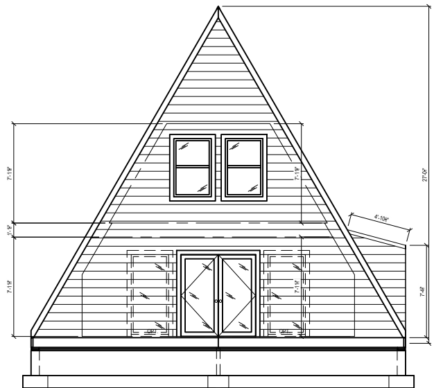
1 FRONT ELEVATION NTS
