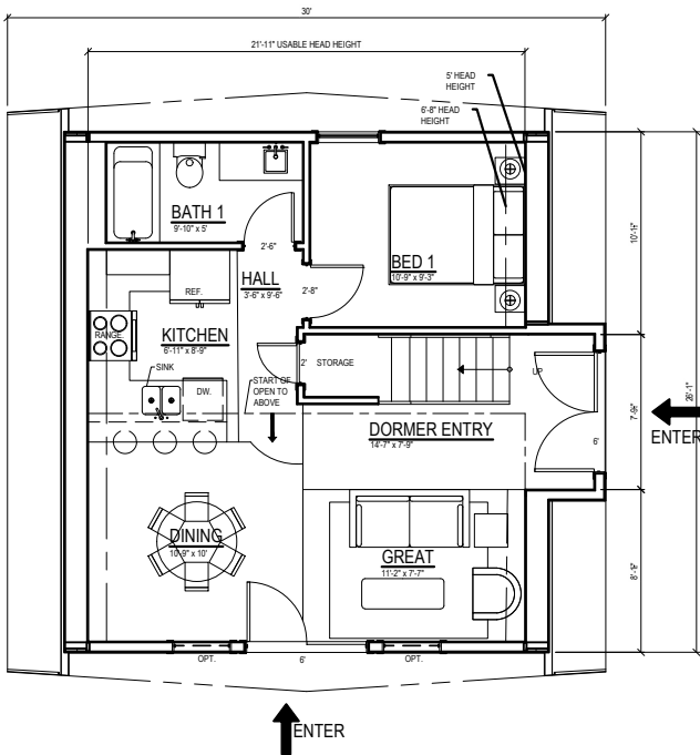
3 MAIN FLOOR PLAN NTS
