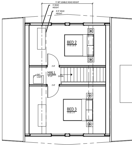
4 UPPER FLOOR PLAN NTS
