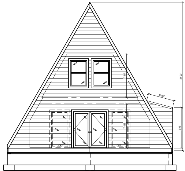
1 FRONT ELEVATION NTS
