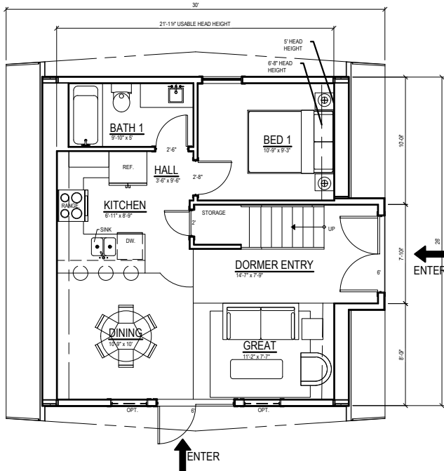
3 MAIN FLOOR PLAN NTS
