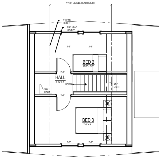
4 UPPER FLOOR PLAN NTS
