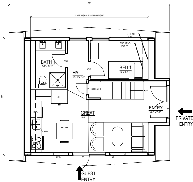
3 MAIN FLOOR PLAN NTS
