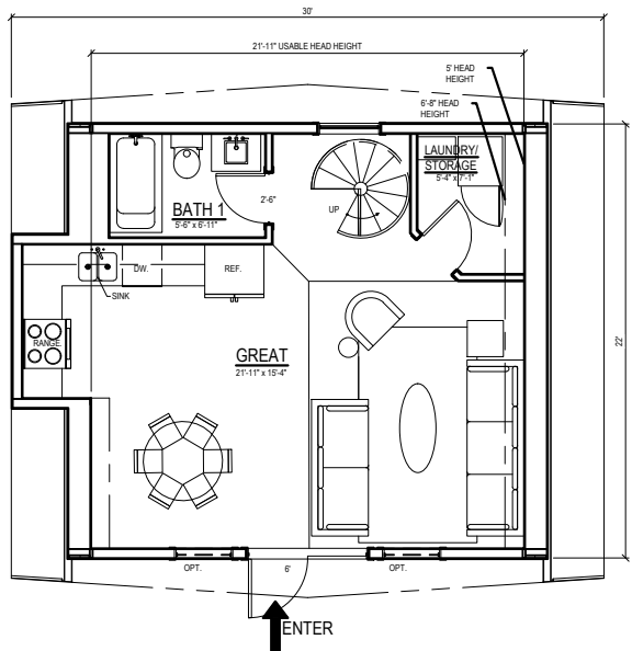
3 MAIN FLOOR PLAN NTS
