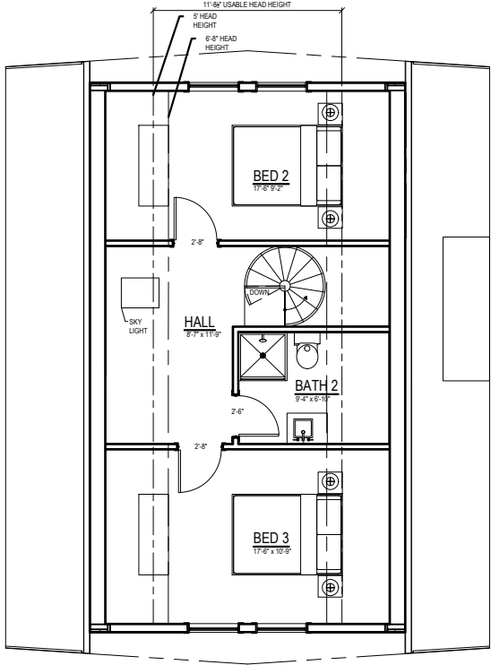
4 UPPER FLOOR PLAN NTS
