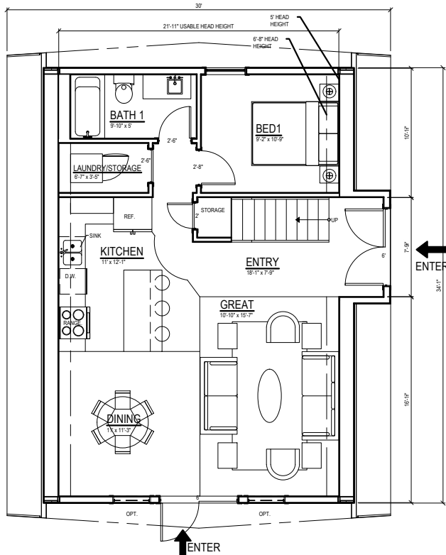
3 MAIN FLOOR PLAN NTS
