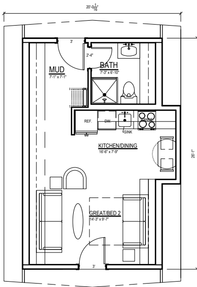
3 FLOOR PLAN NTS
