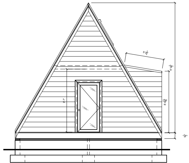
1 FRONT ELEVATION NTS
