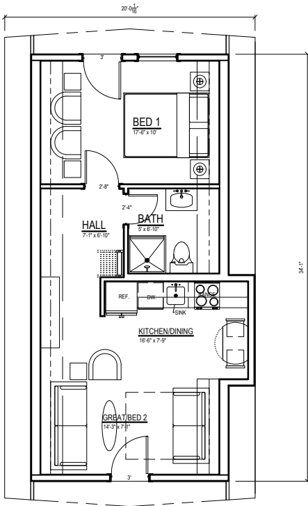
3 FLOOR PLAN NTS
