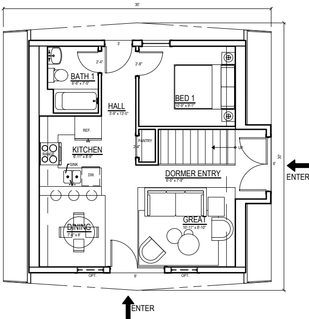
4 UPPER FLOOR PLAN NTS
