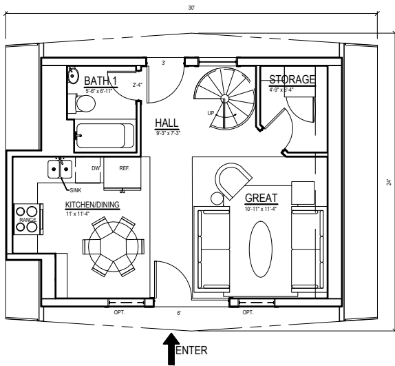
3 MAIN FLOOR PLAN NTS
