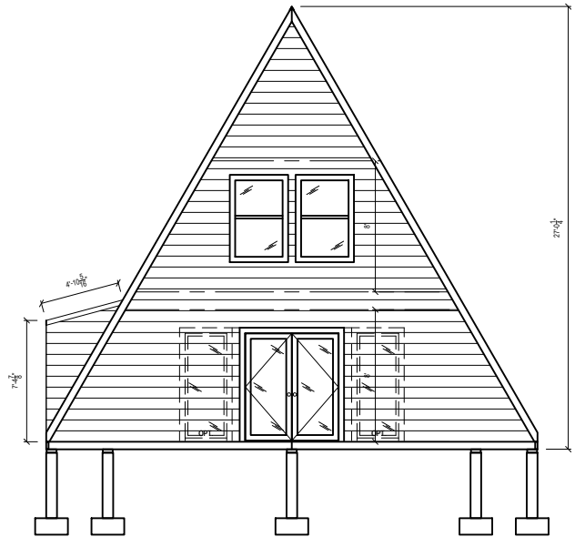
1 FRONT ELEVATION NTS
