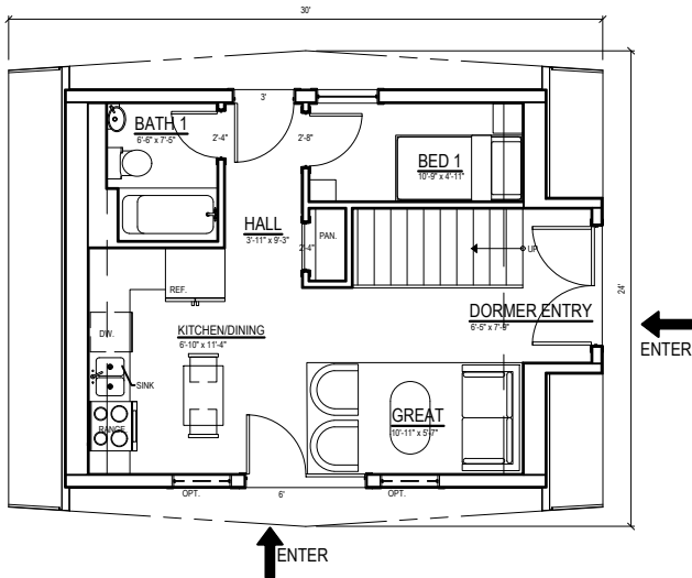
3 MAIN FLOOR PLAN NTS
