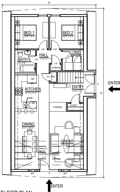
3 MAIN FLOOR PLAN NTS
