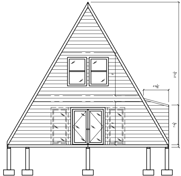
1 FRONT ELEVATION NTS
