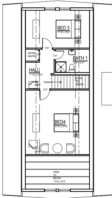
4 UPPER FLOOR PLAN NTS
