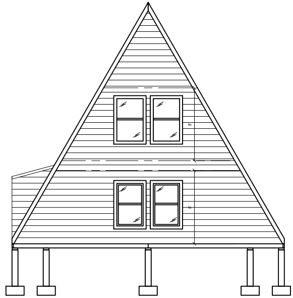
2 REAR ELEVATION NTS
