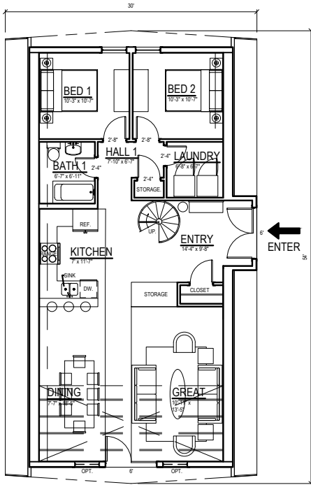
3 MAIN FLOOR PLAN NTS
