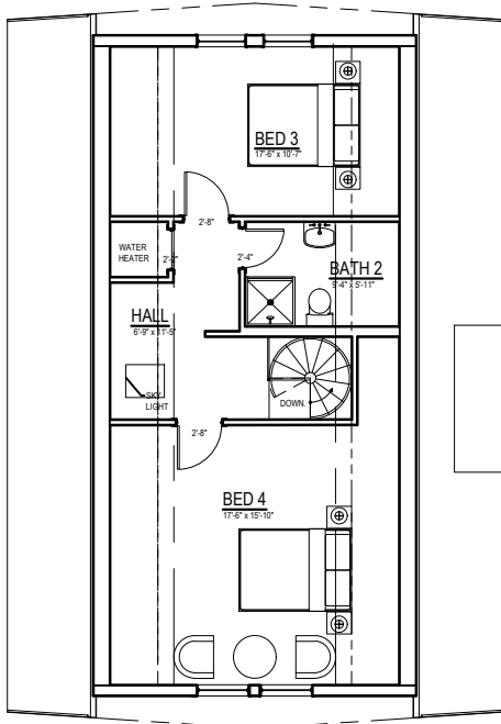
4 UPPER FLOOR PLAN NTS
