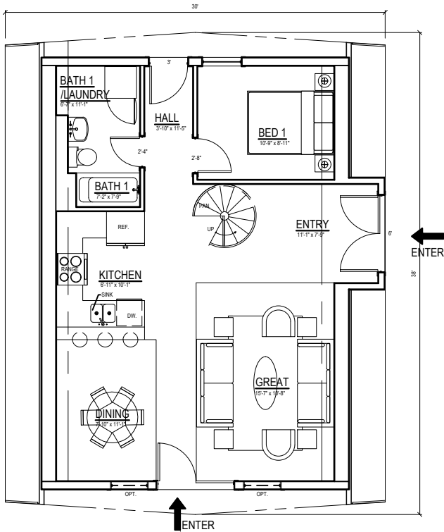
3 MAIN FLOOR PLAN NTS
