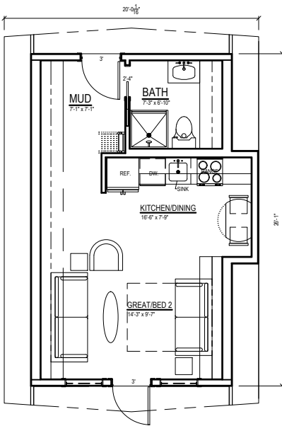
3 FLOOR PLAN NTS
