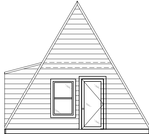
2 REAR ELEVATION NTS
